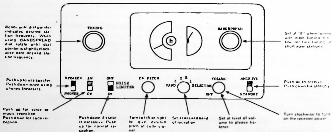
Figure 5. Radio Receiver Model S-38, view showing use of controls.
