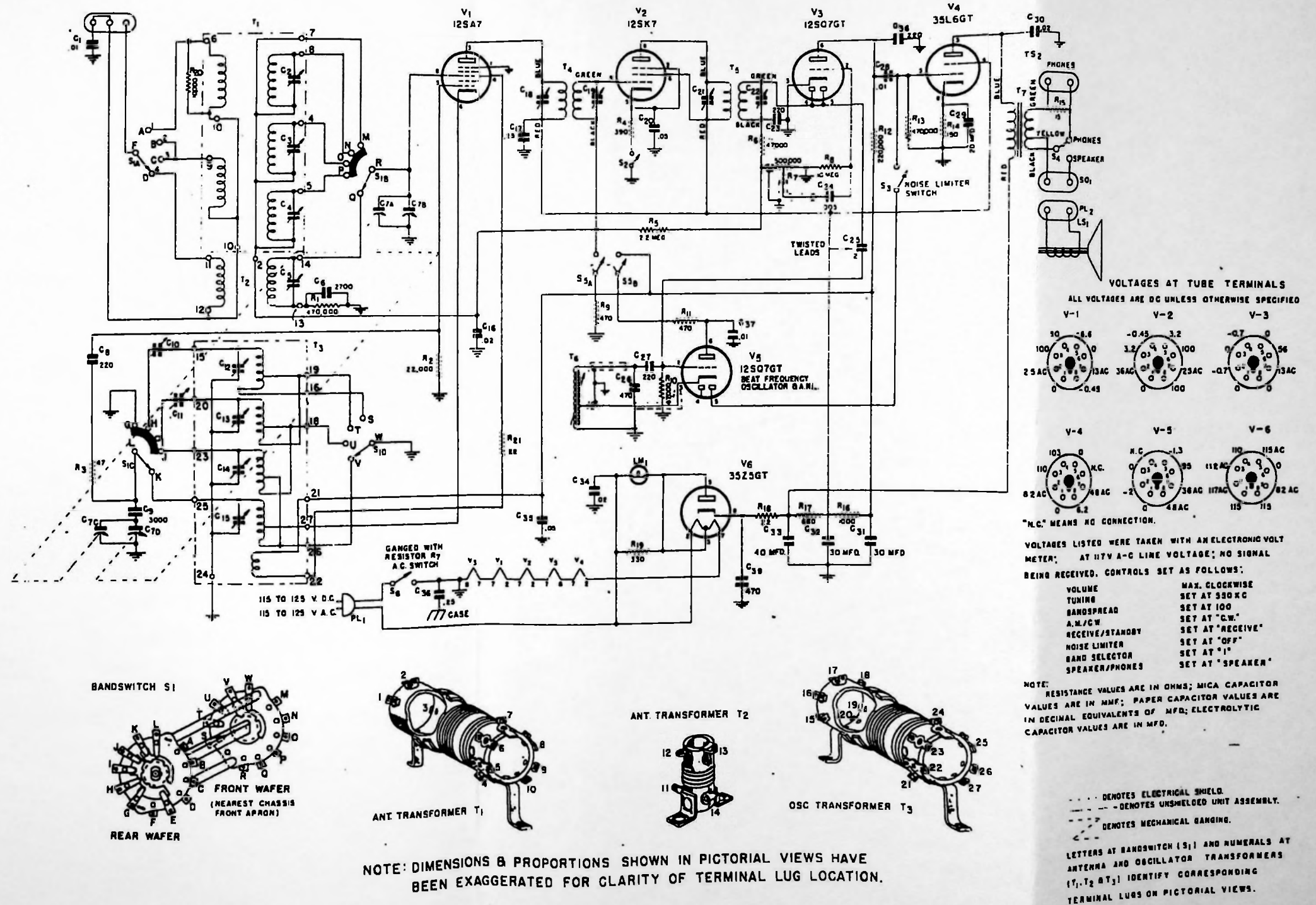
Fig. 3 Schematic diagram including tube terminal voltages and pictorial views of bandswitch, mixer and oscillator coil forms for terminal lug location and cross reference to the schematic.
