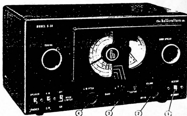
Fig. 1. Front view of receiver showing control locations.
