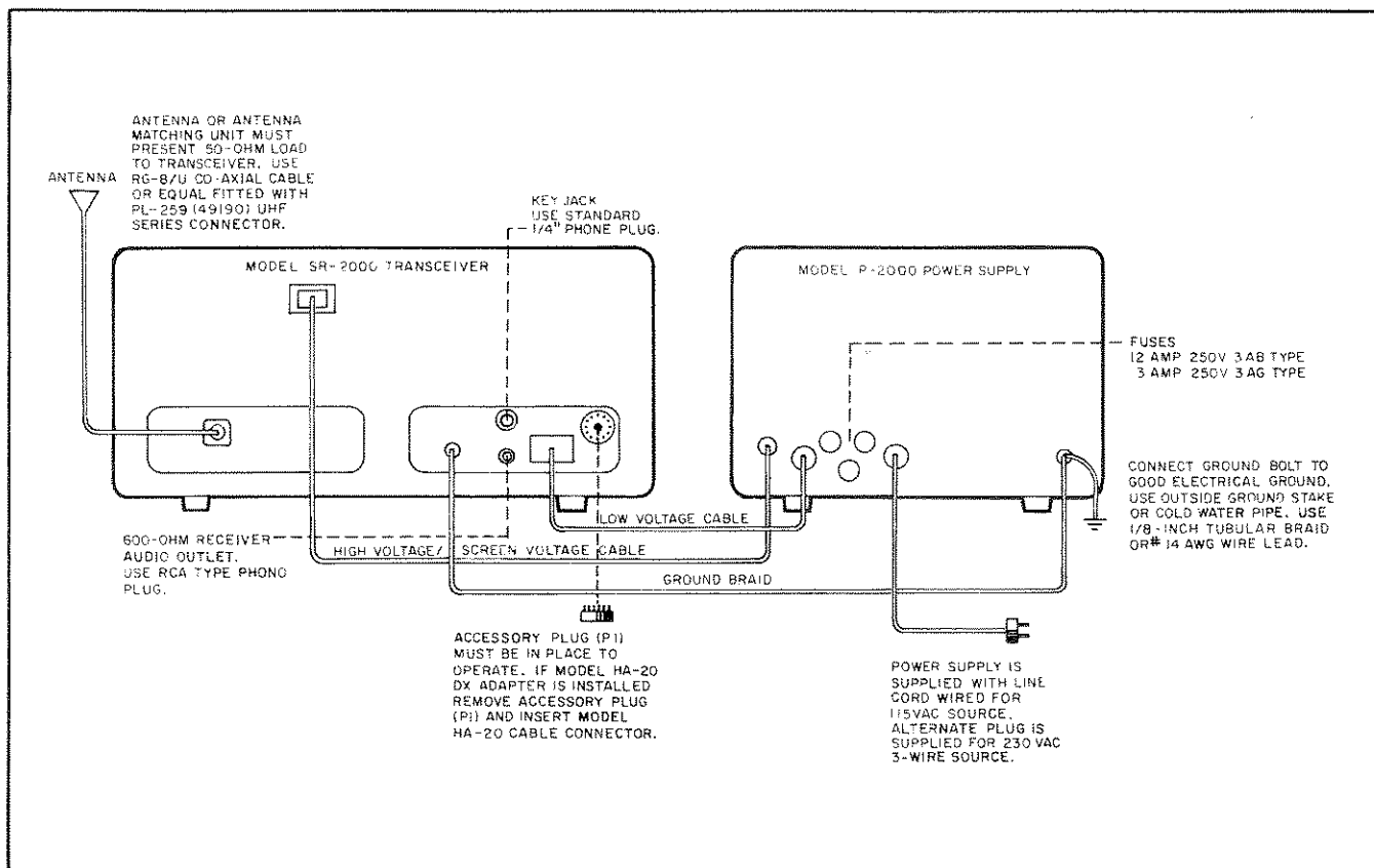
Figure 5. Typical Installation.
