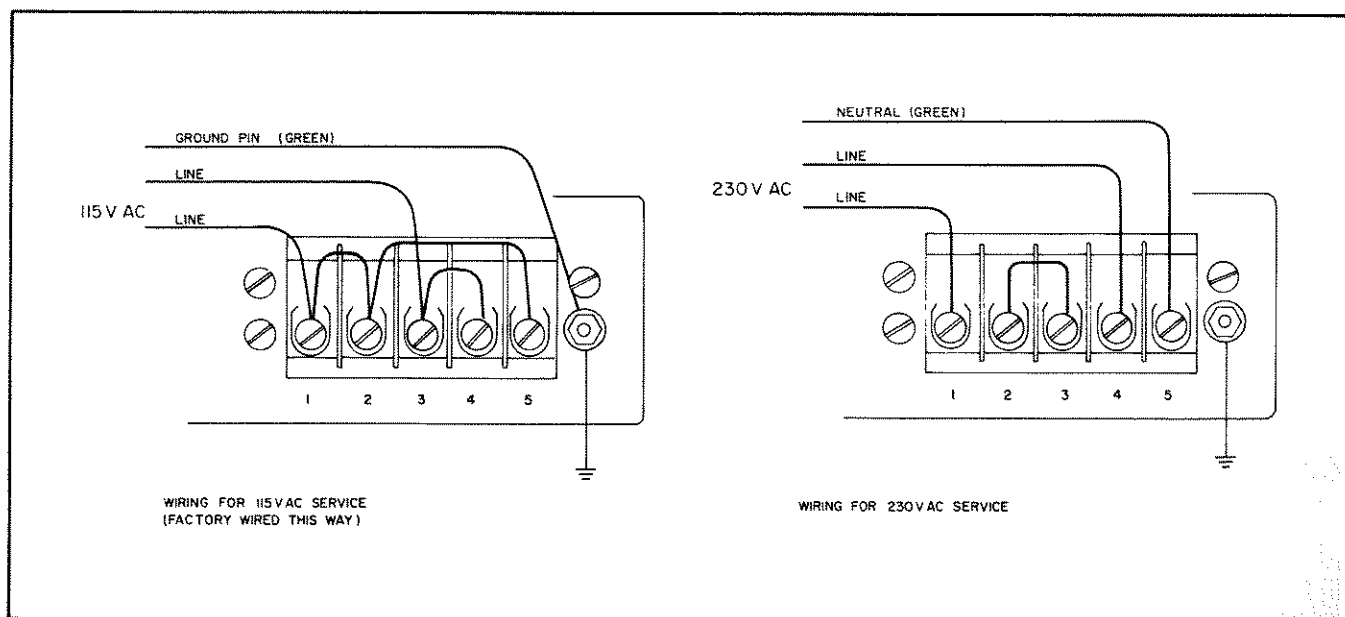
Figure 18. Model P-2000 Power Supply, Primary Power Connections.
