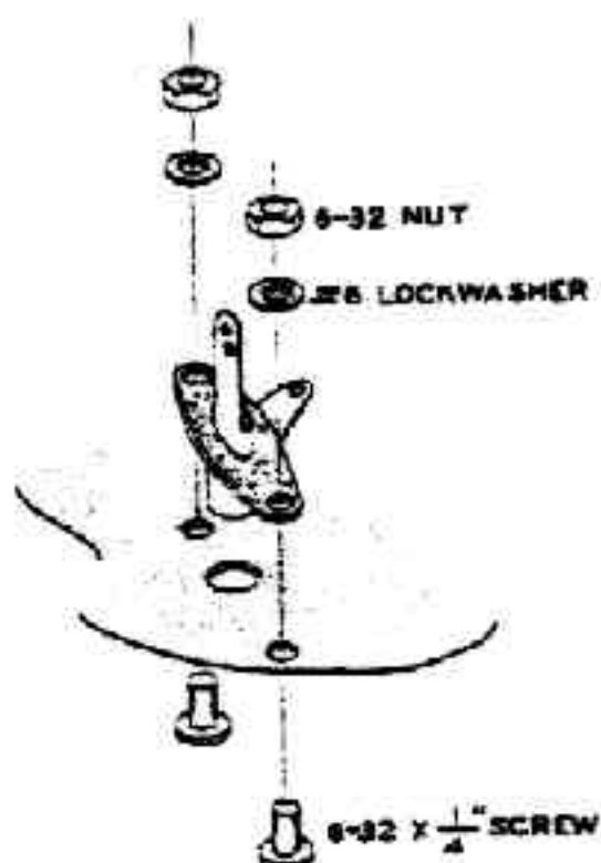
Detail 1G
