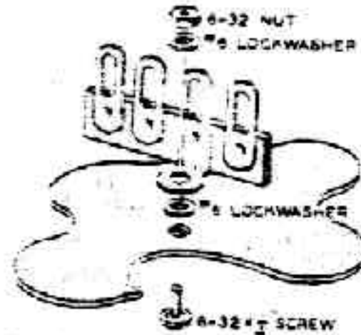
Detail 1D
