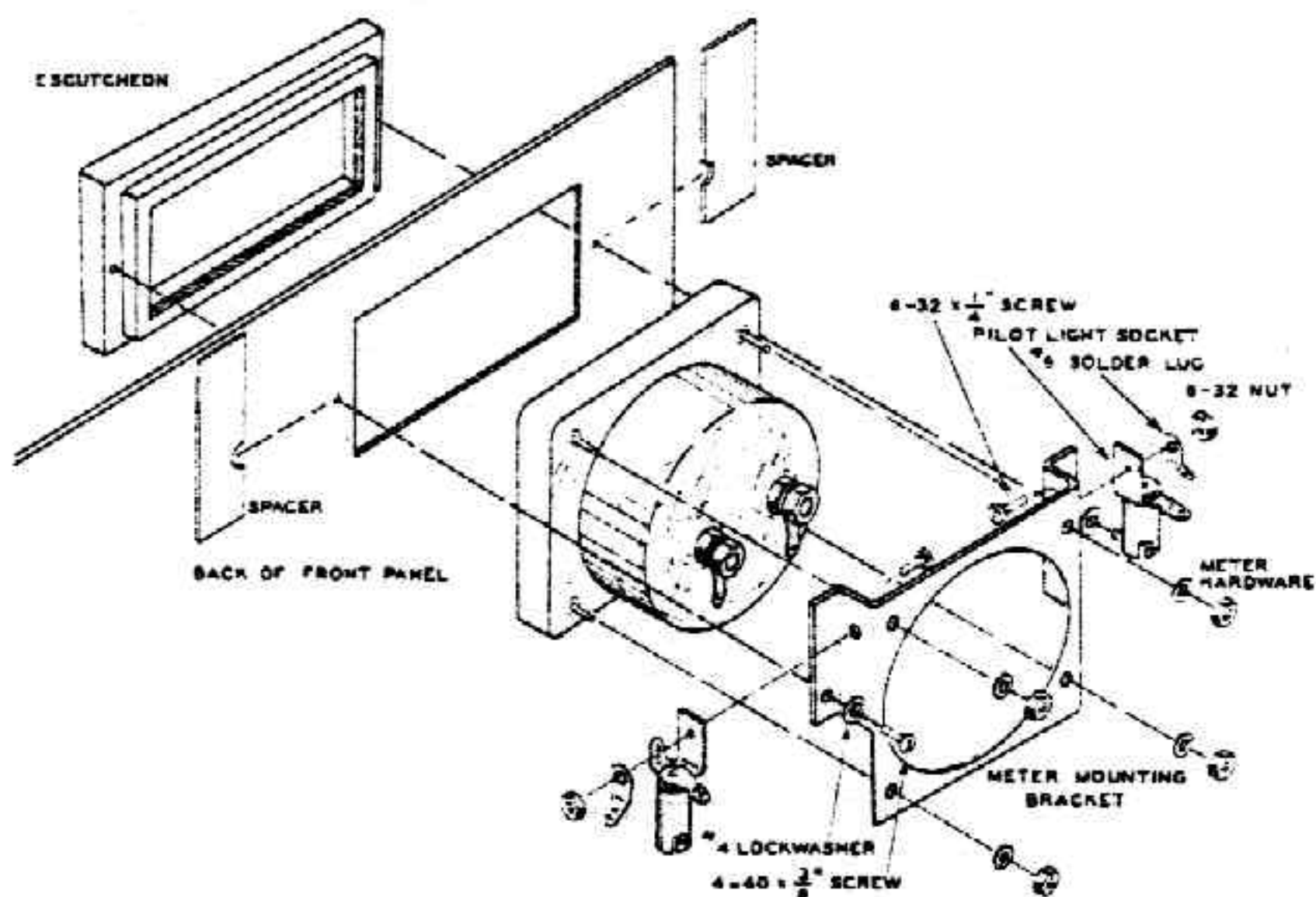
Detail 4B
