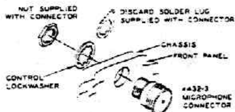
Detail 1H
