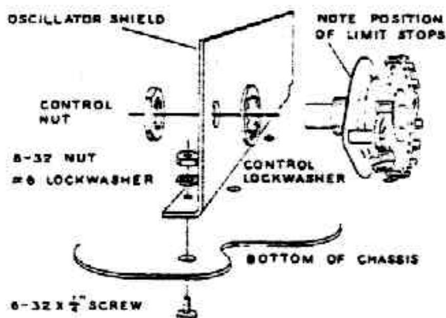
Detail 3F
