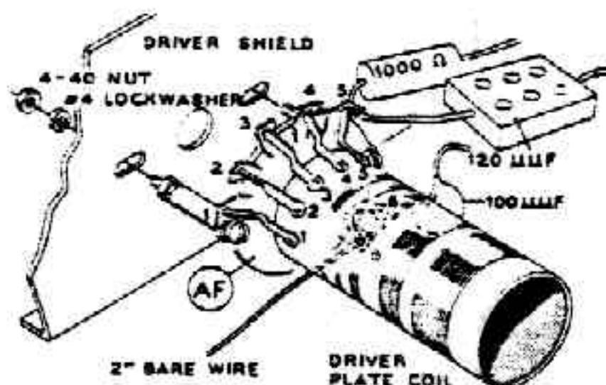
Detail 6A
