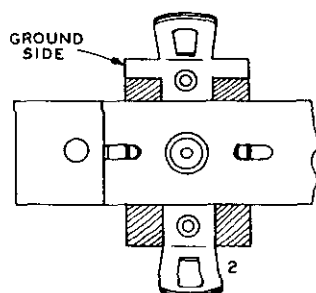
TRIMMER CAPACITOR
