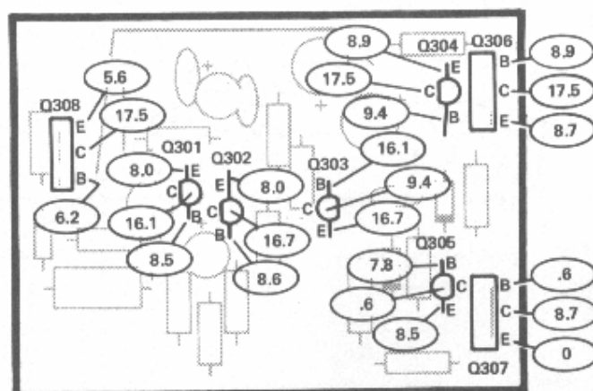
AUDIO CIRCUIT BOARD (Shown from component side)
