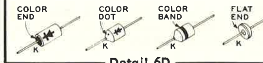
Detail 6D
