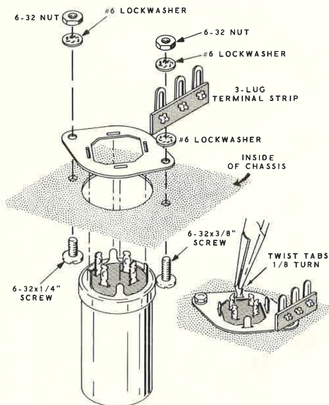
Detail 4H
