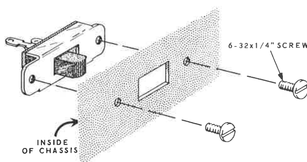
Detail 4C
