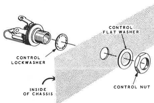
Detail 4B
