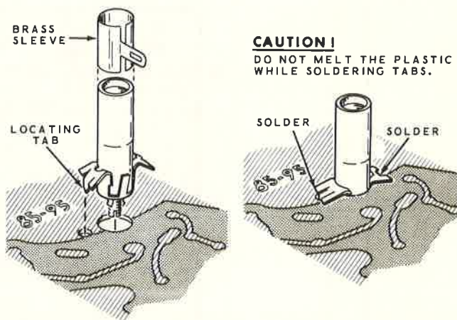
Detail 8A
