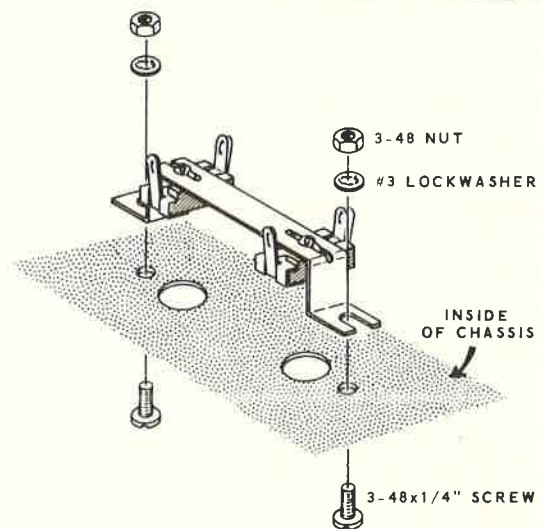
Detail 4F
