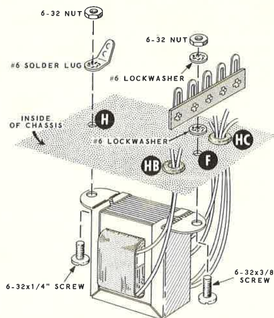
Detail 4J
