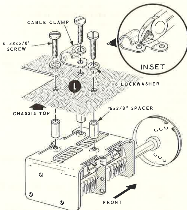
Detail 6B
