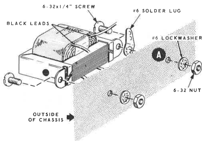
Detail 4A
