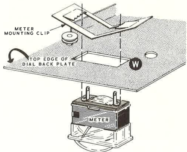
Detail 5A
