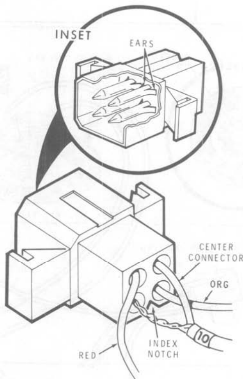
Detail 12-29B
