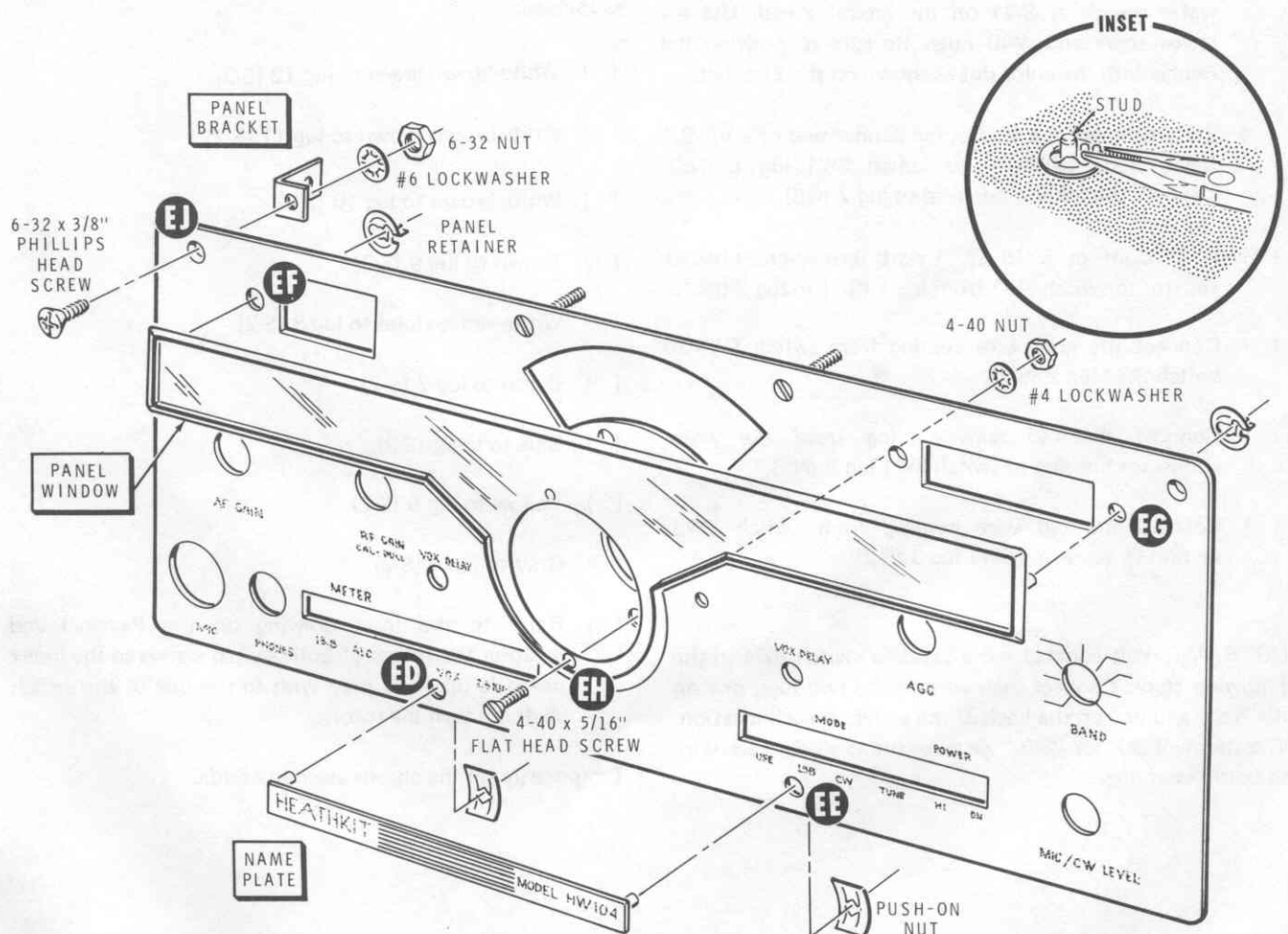
Detail 12-31C
