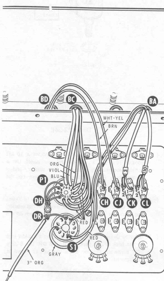
PICTORIAL 12-25
