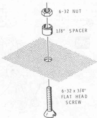
Detail 12-31A
