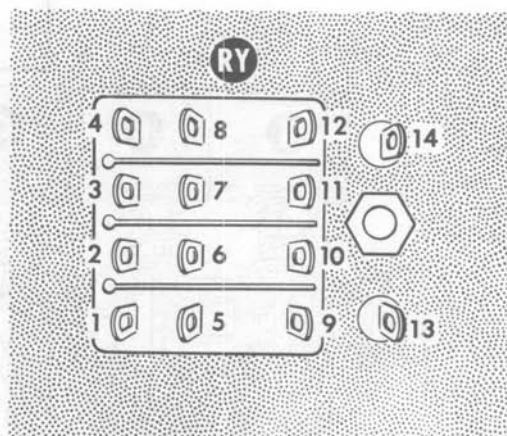
Detail 12-7A
