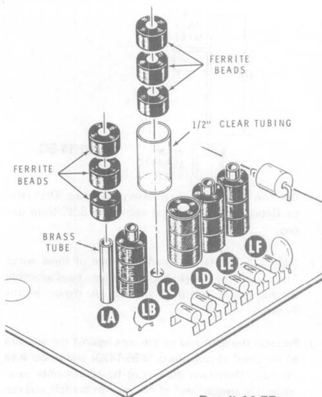
Detail 11-5B
