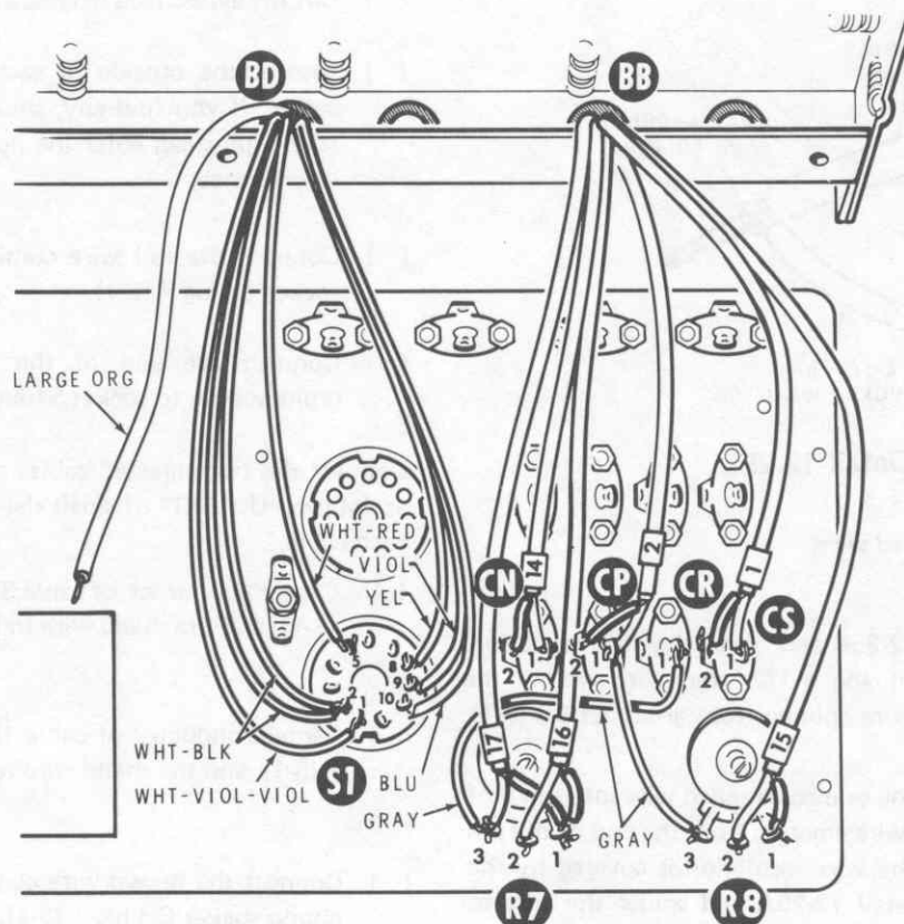
PICTORIAL 12-26
