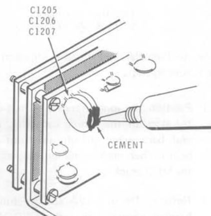
Detail 1-11D
