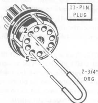
Detail 12-27A
