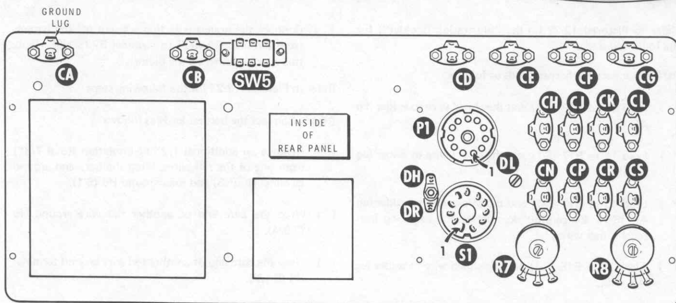
PICTORIAL 12-24
