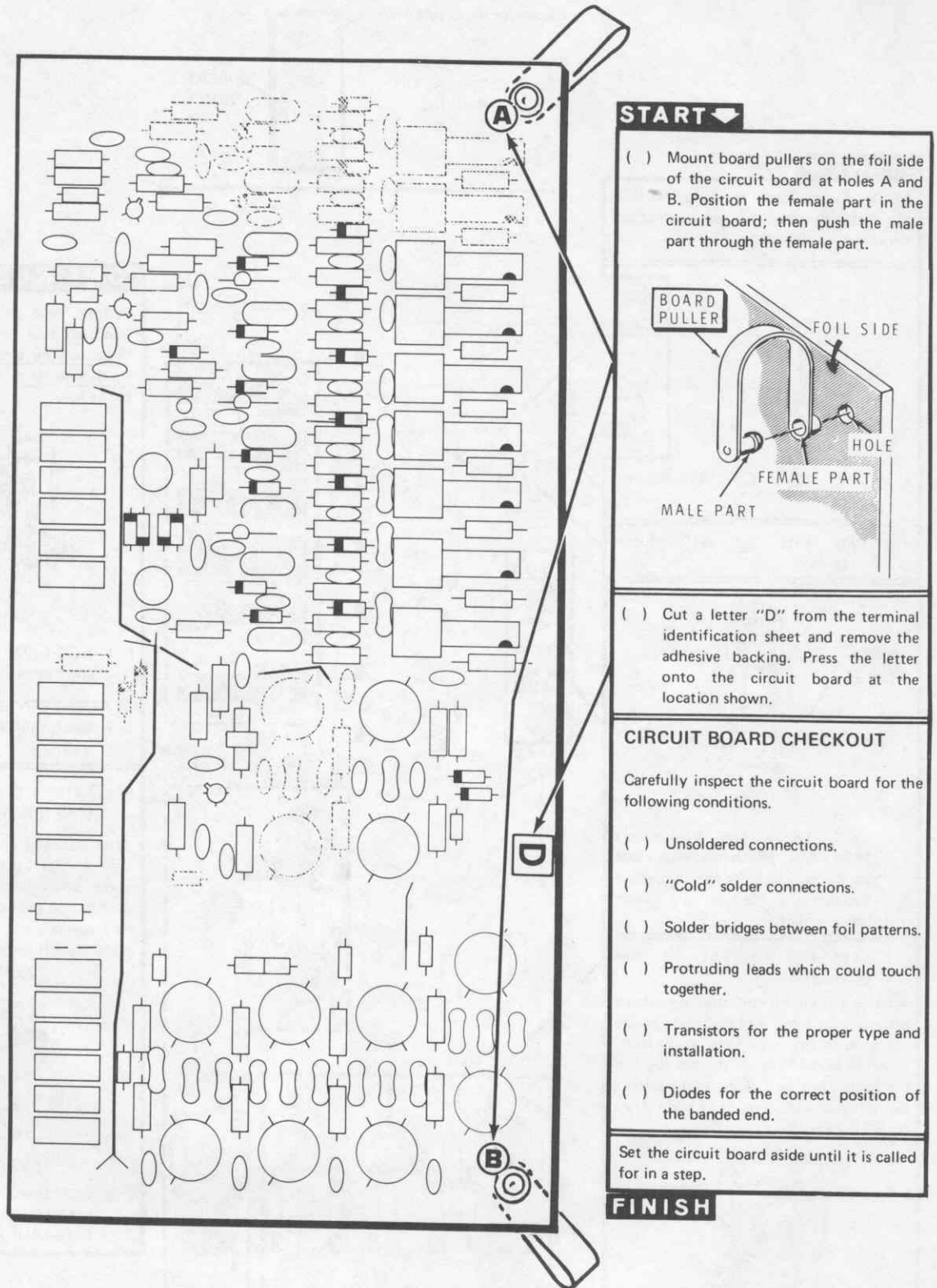
PICTORIAL 3-9
