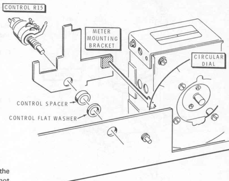
Detail 12-32D
