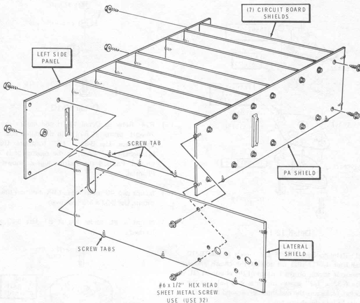
Detail 12-2A
