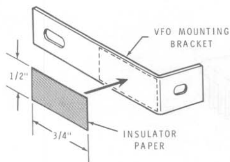
Detail 12-32M
