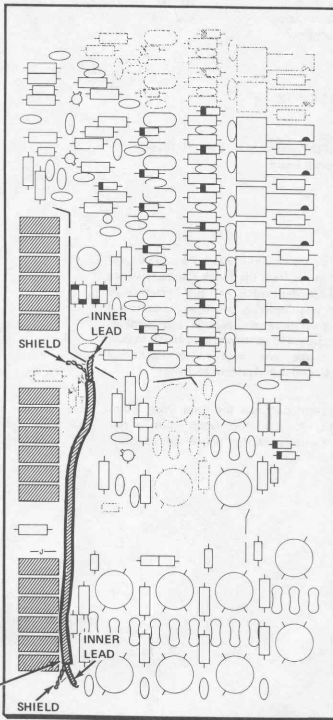
PICTORIAL 3-1
