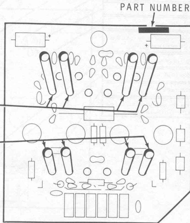
PICTORIAL 114
