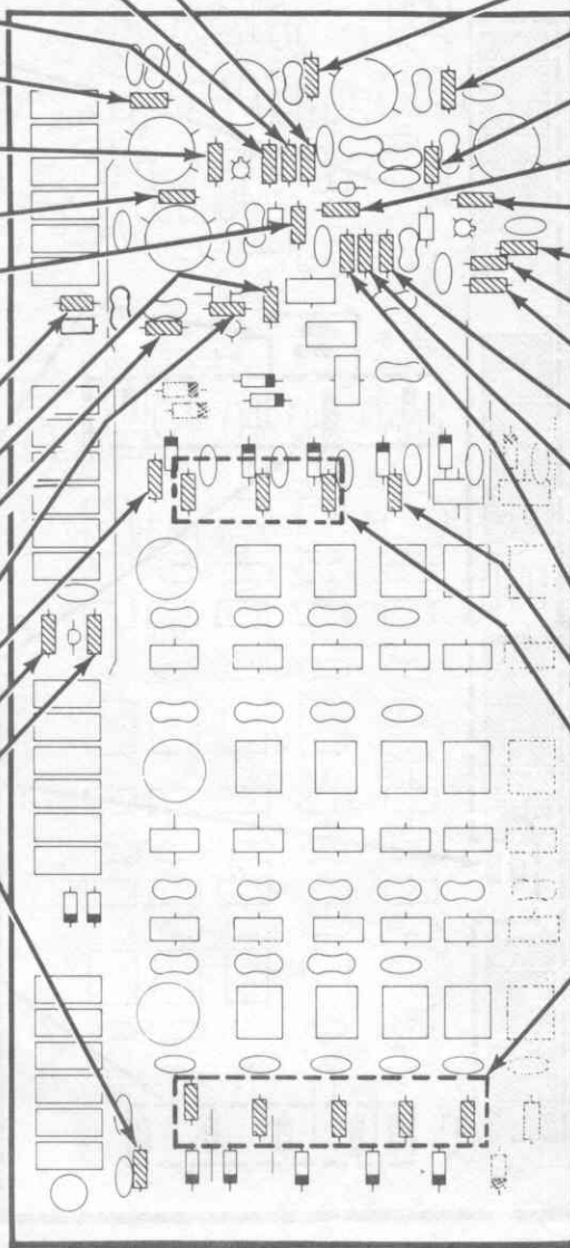
PICTORIAL 9-2
