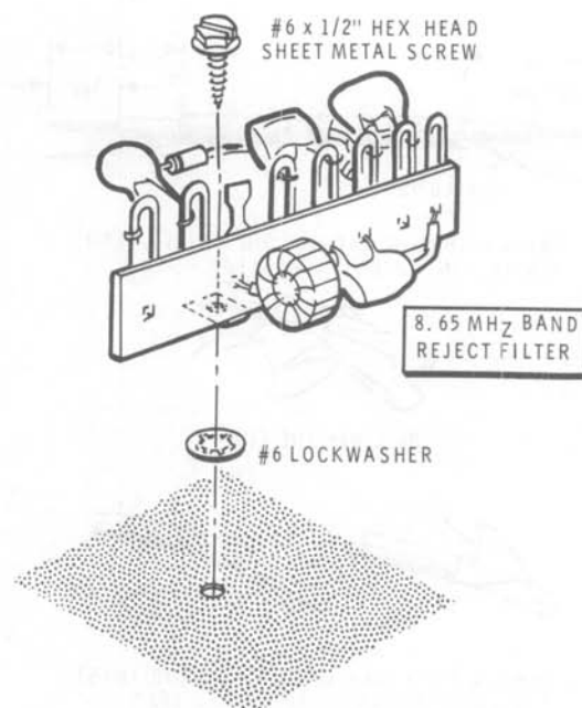
Detail 12-19B
