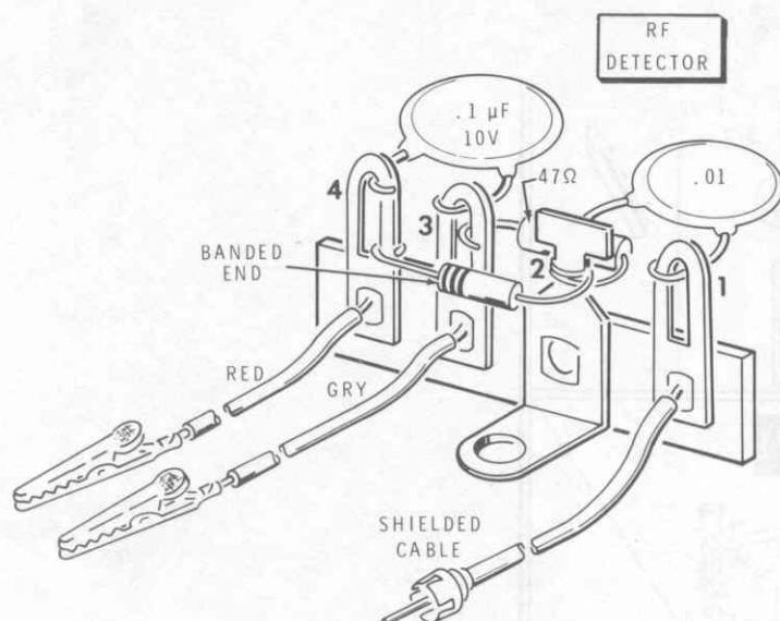
PICTORIAL 12-36
