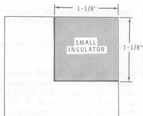
Detail 1-10B
