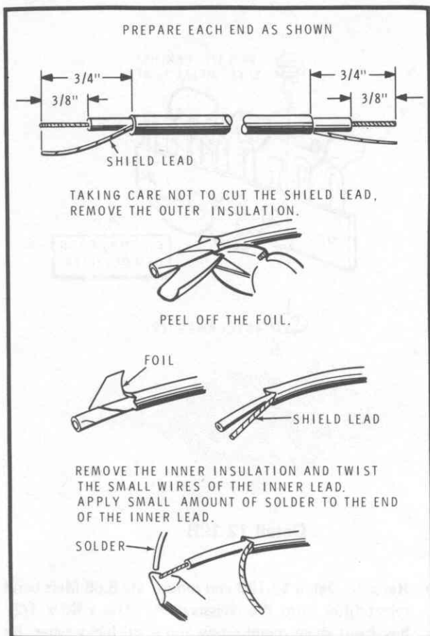
Detail 12-19C
