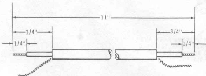
Detail 12-21A
