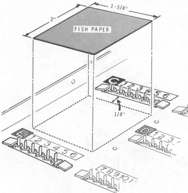
Detail 12-1D
