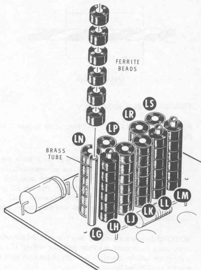
Detail 11-5D
