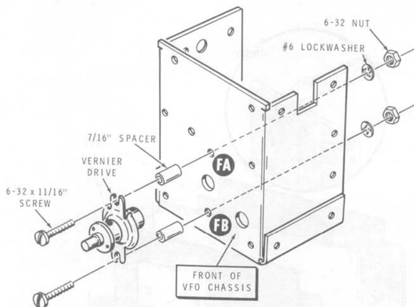
PICTORIAL 1-9
