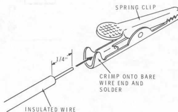
Detail 12-36B
