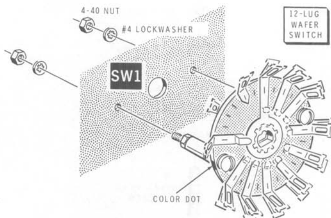
Detail 12-30B
