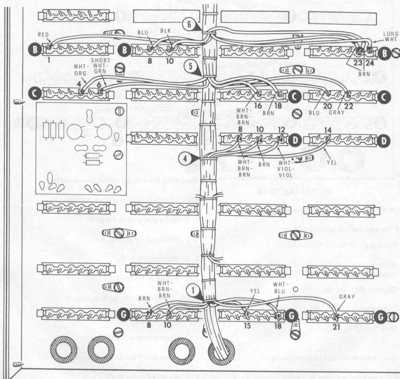
PICTORIAL 12-17
