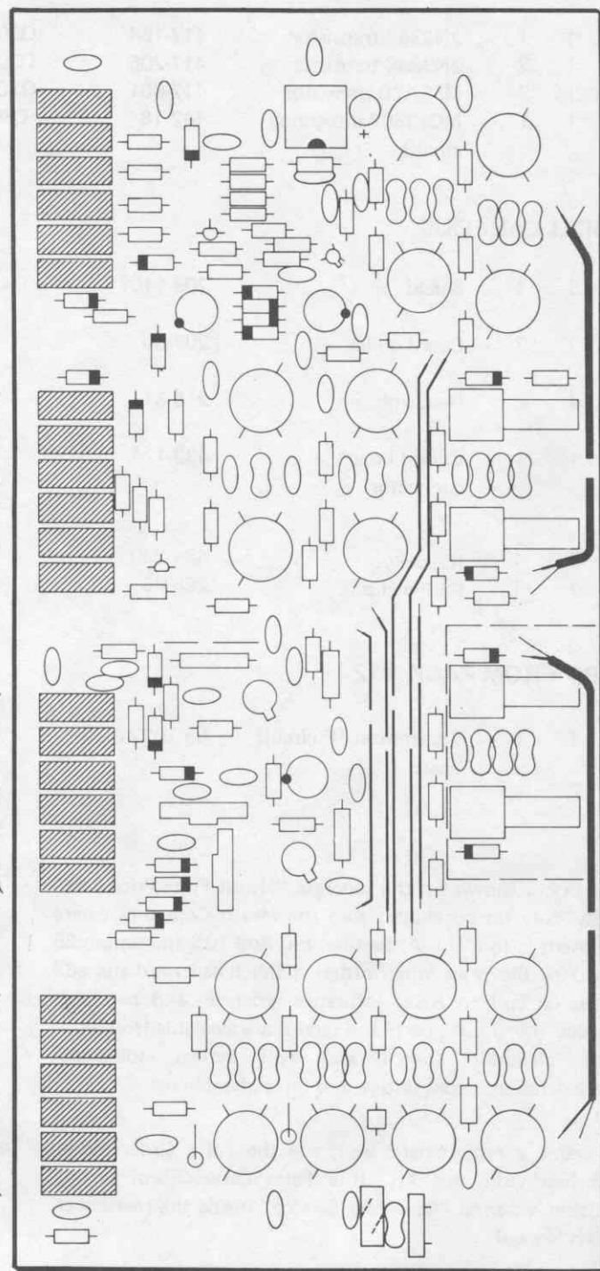
PICTORIAL 5-1
