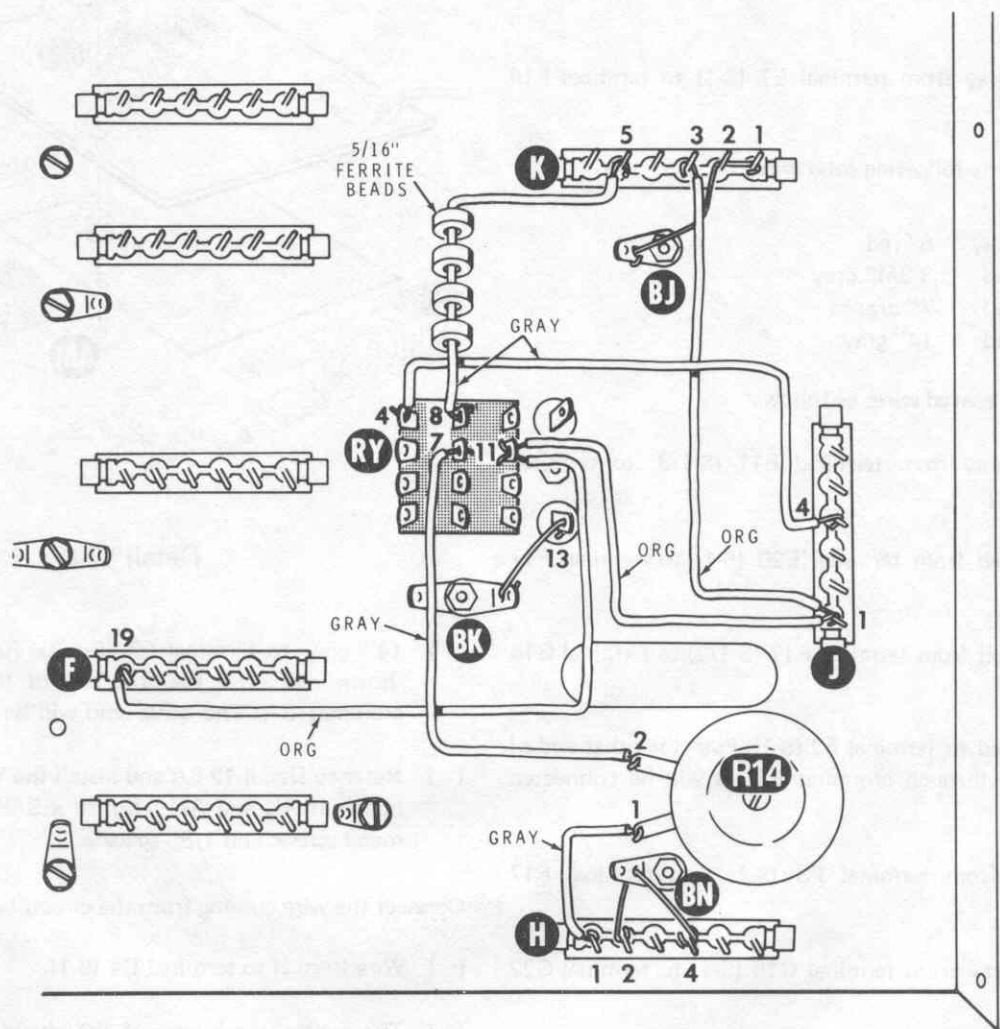
PICTORIAL 12-7
