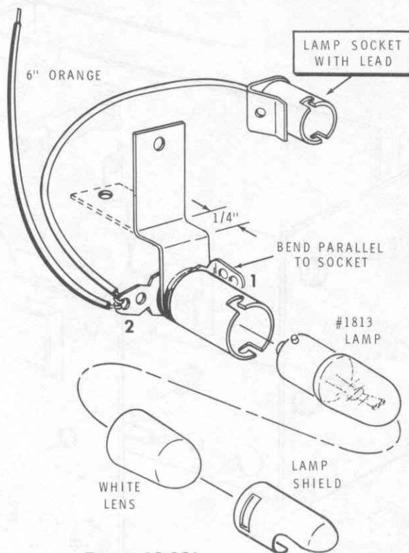
Detail 12-32L
