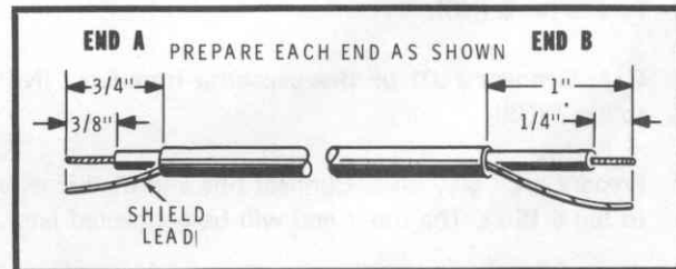
Detail 12-19D
