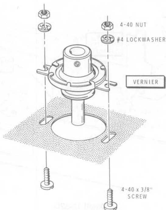
Detail 12-31H
