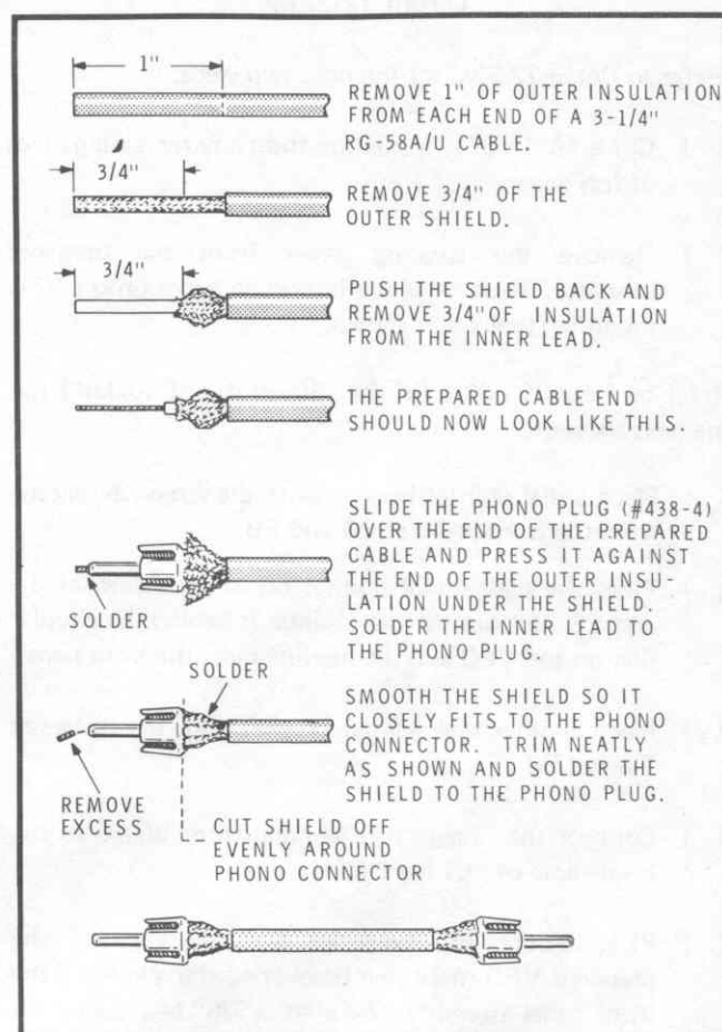
Detail 12-33B
