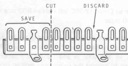
Detail 12-36A
