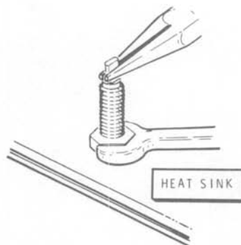
Detail 11-11B
