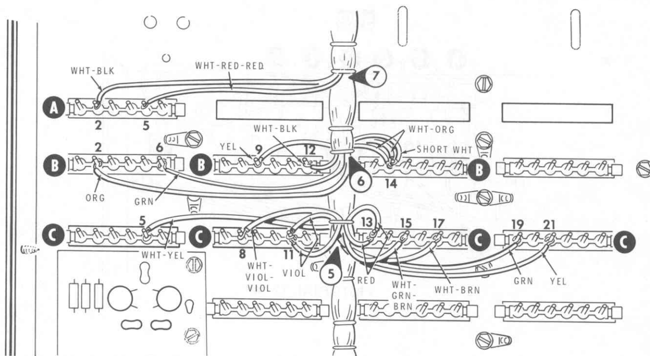
PICTORIAL 12-15
