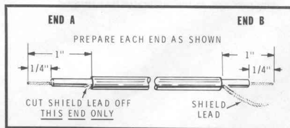
Detail 12-36C
