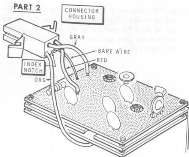
Detail 1-12D
