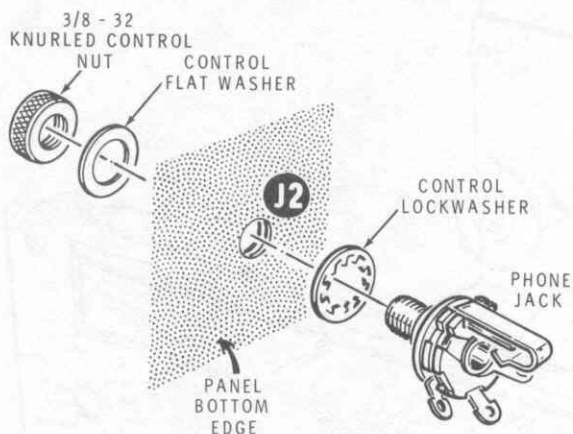
Detail 12-32H
