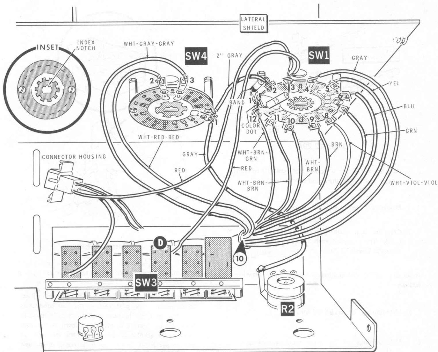
PICTORIAL 12-30
