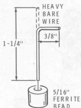
Detail 11-5C
