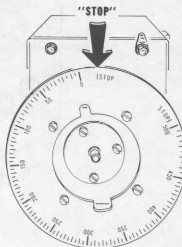
Detail 1-15A
