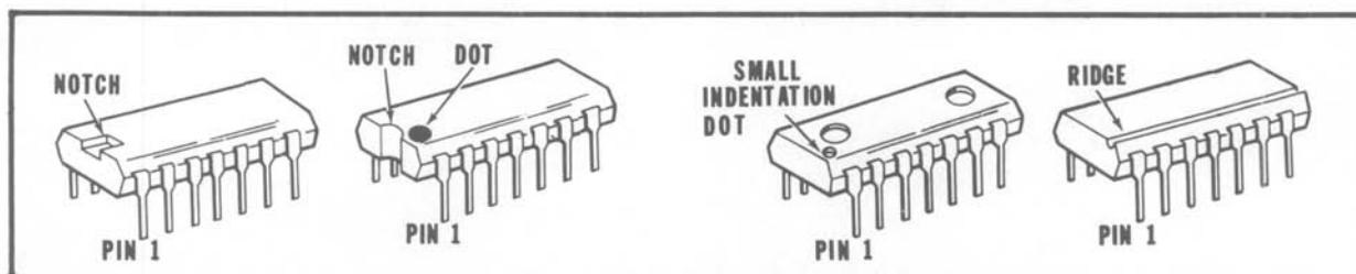
Detail 4-3A
