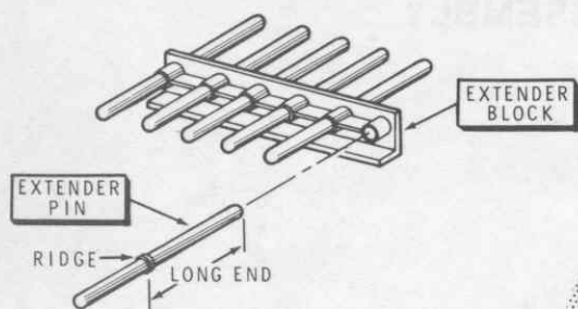
PICTORIAL 1-2A
