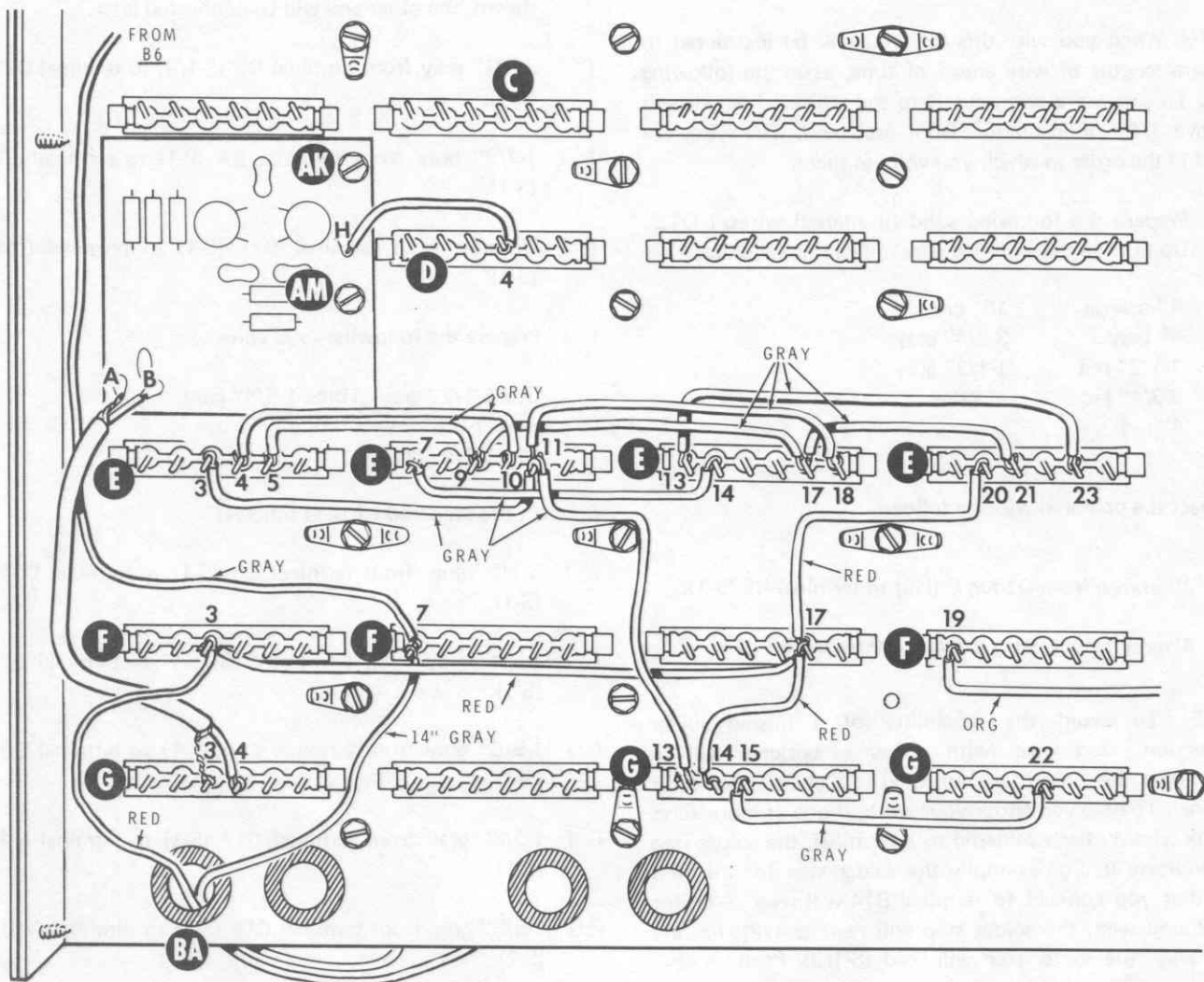
PICTORIAL 12-6
