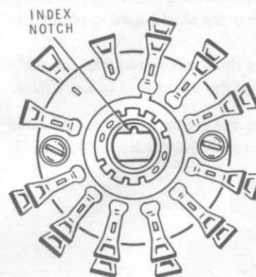
Detail 12-35B
