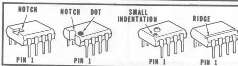
Detail 5-10A
