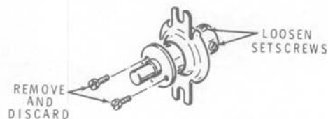
Detail 1-9A
