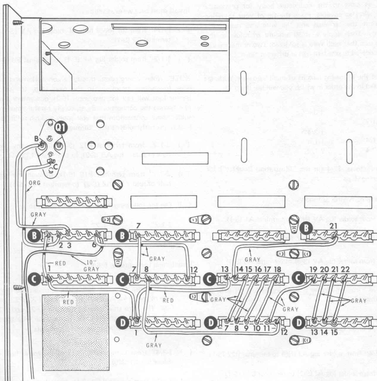
PICTORIAL 12-5
