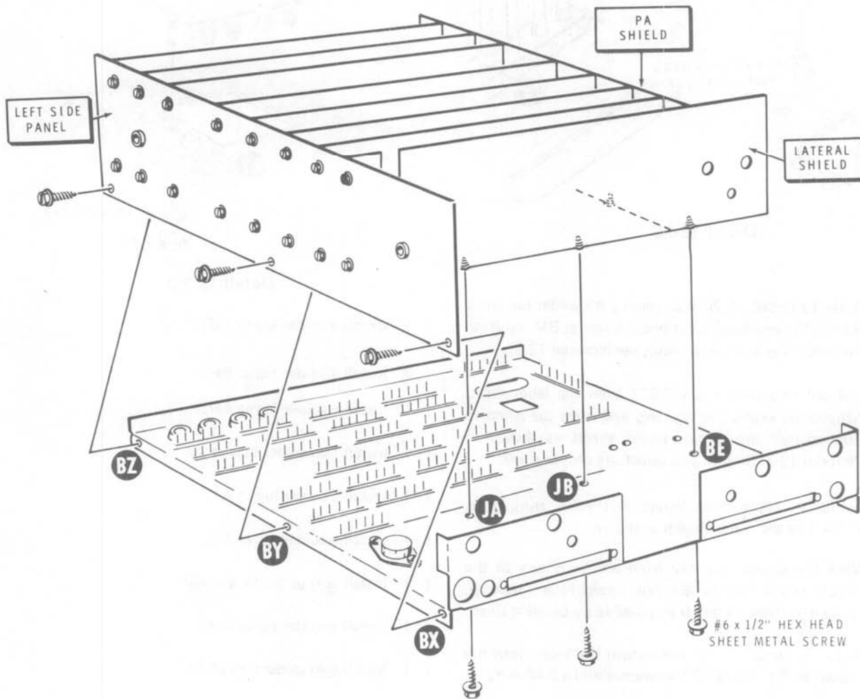
Detail 12-2B
