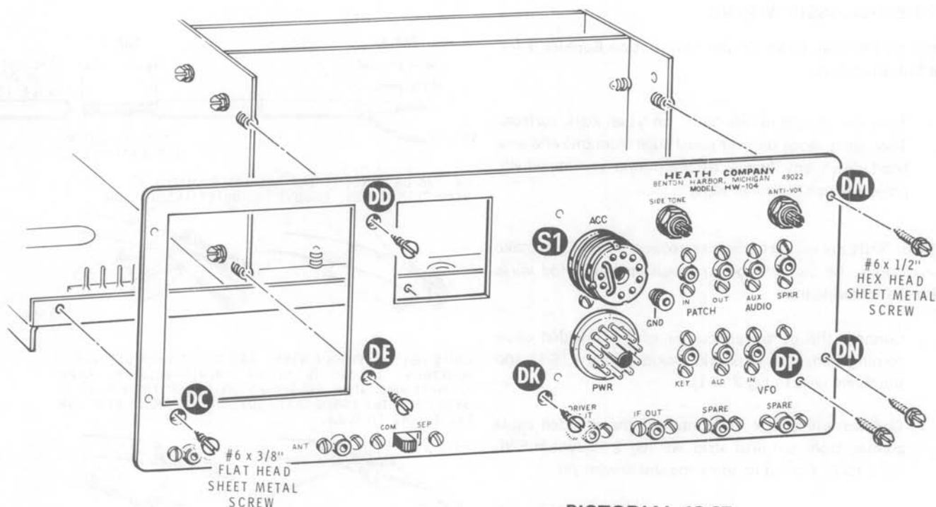
PICTORIAL 12-27
