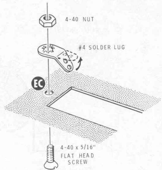
Detail 12-31B
