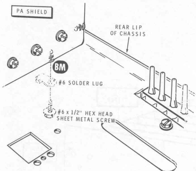
Detail 12-2C
