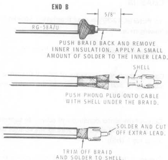
Detail 12-28C
