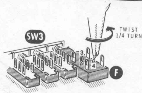
Detail 12-21B
