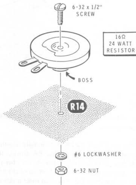
Detail 12-1H
