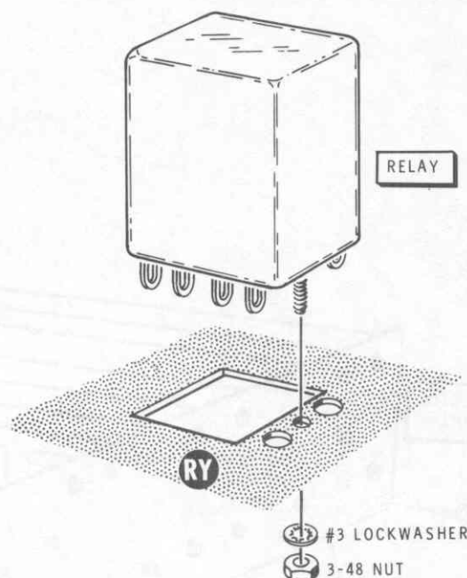
Detail 12-2D
