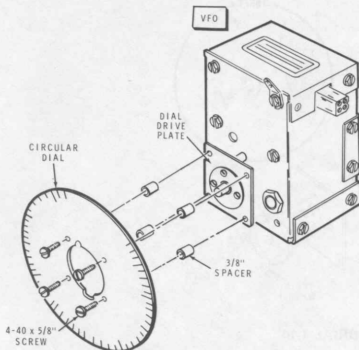
PICTORIAL 1-15
