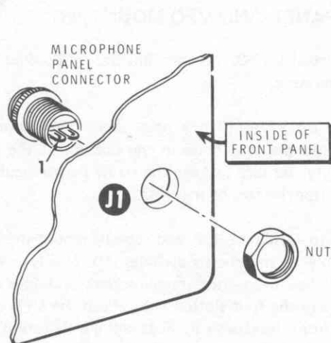
Detail 12-32B
