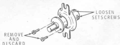
Detail 12-31G
