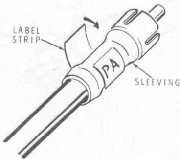
Detail 12-28G
