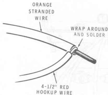
Detail 12-25B
