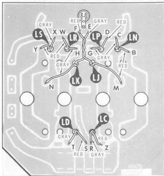
PICTORIAL 11-6
