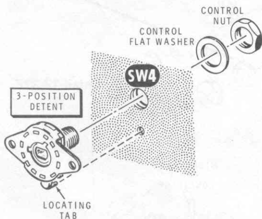
Detail 12-32J
