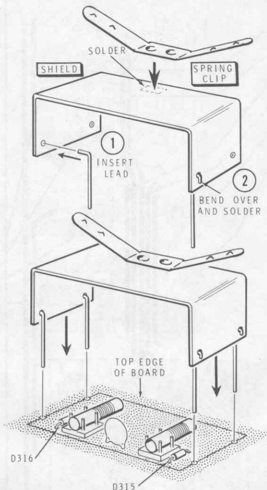
PICTORIAL 5-13
