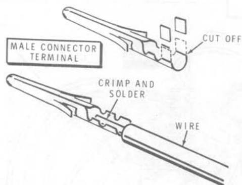
Detail 12-29A
