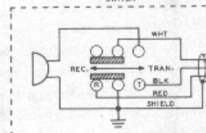
MICROPHONE WITH PUSH-TO-TALK SWITCH
