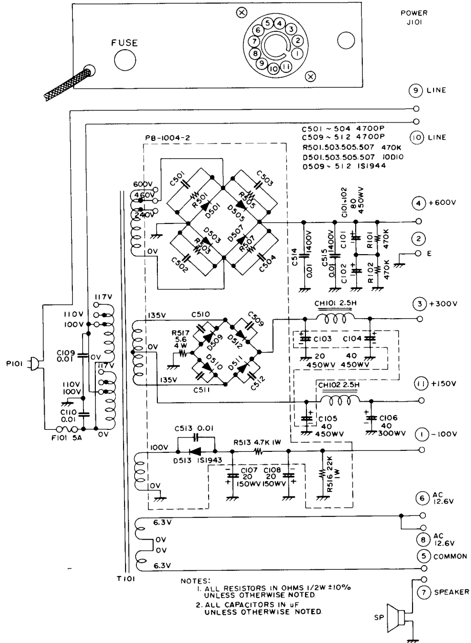
POWER SUPPLY
