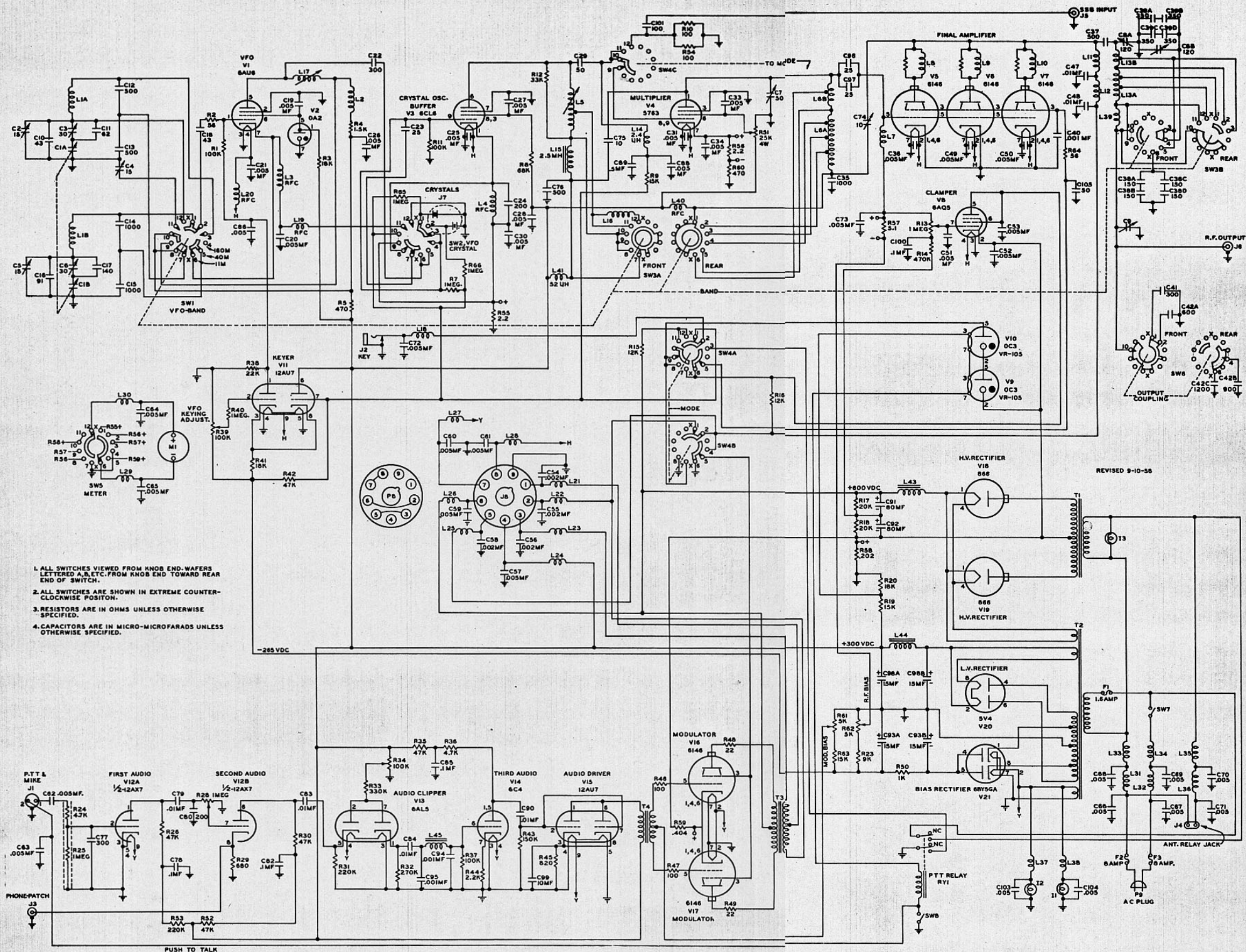
Figure 9, Valiant Schematic Diagram
