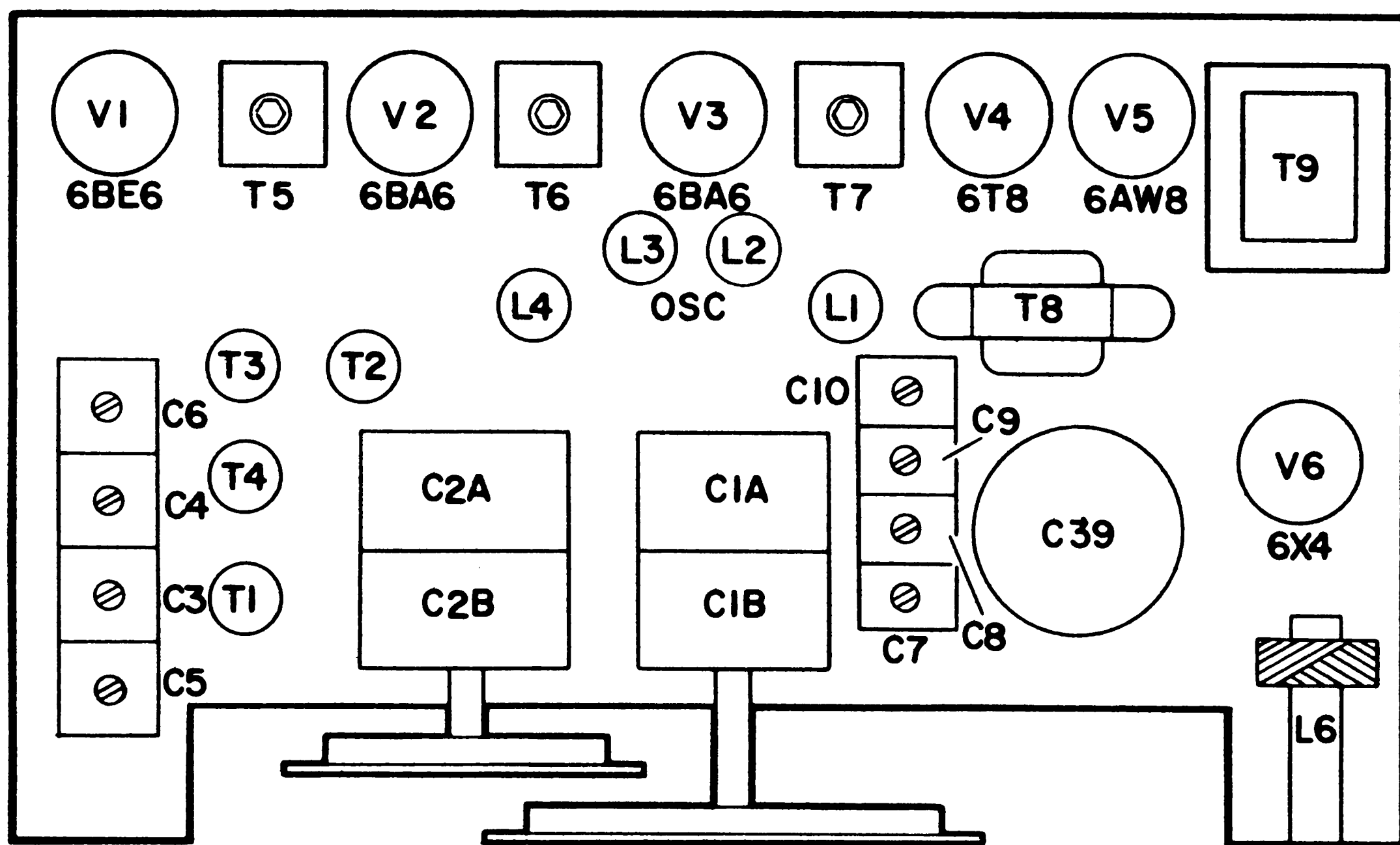
Alignment Locations
