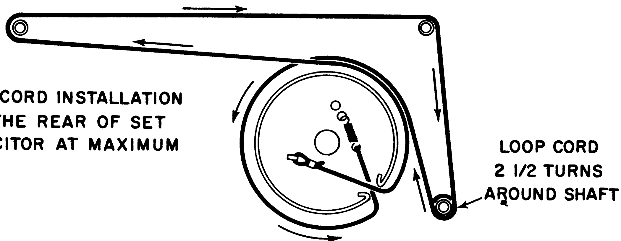
Dial Cord Assembly
