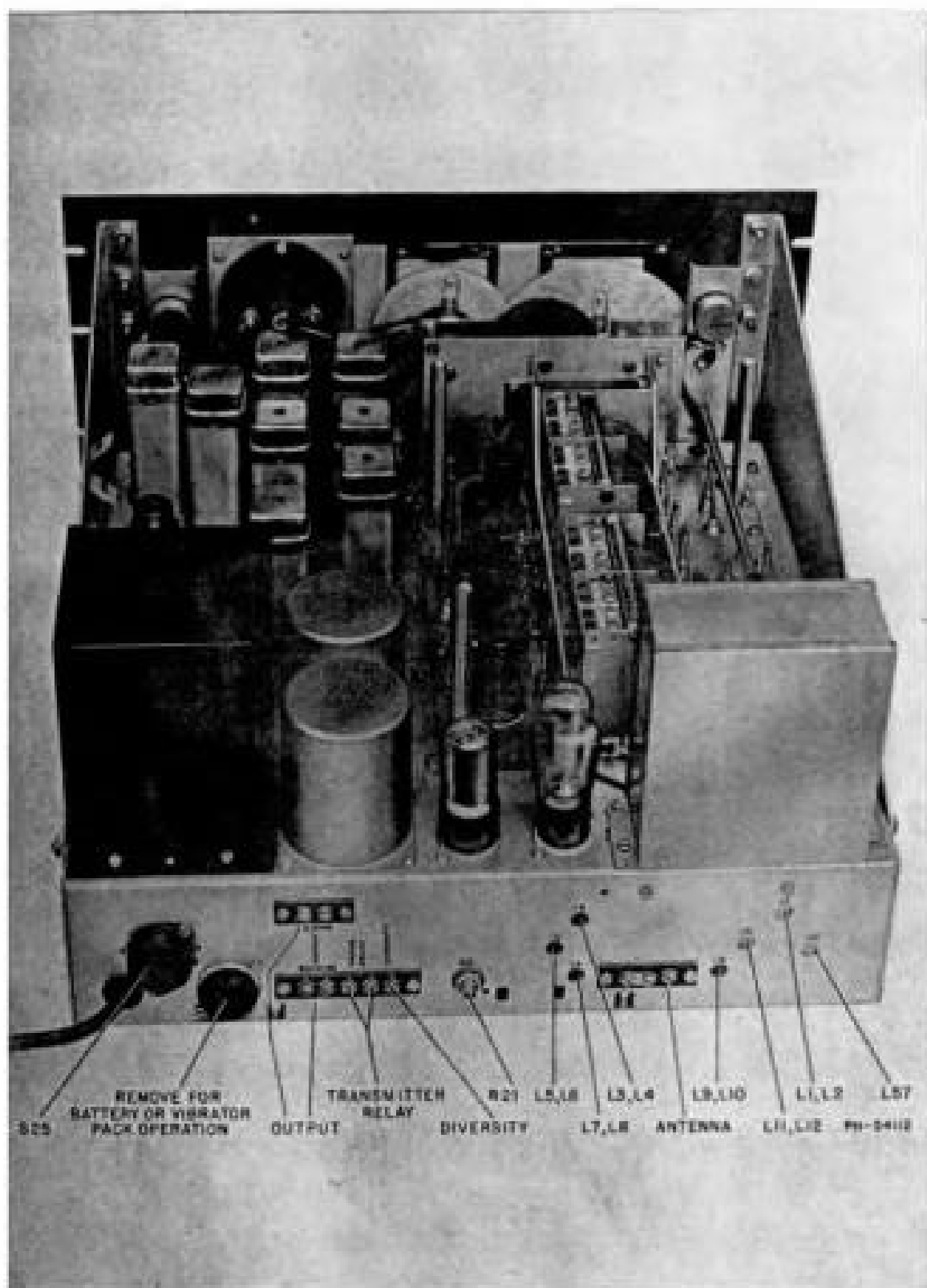
Figure 6—AR-88 Chassis
