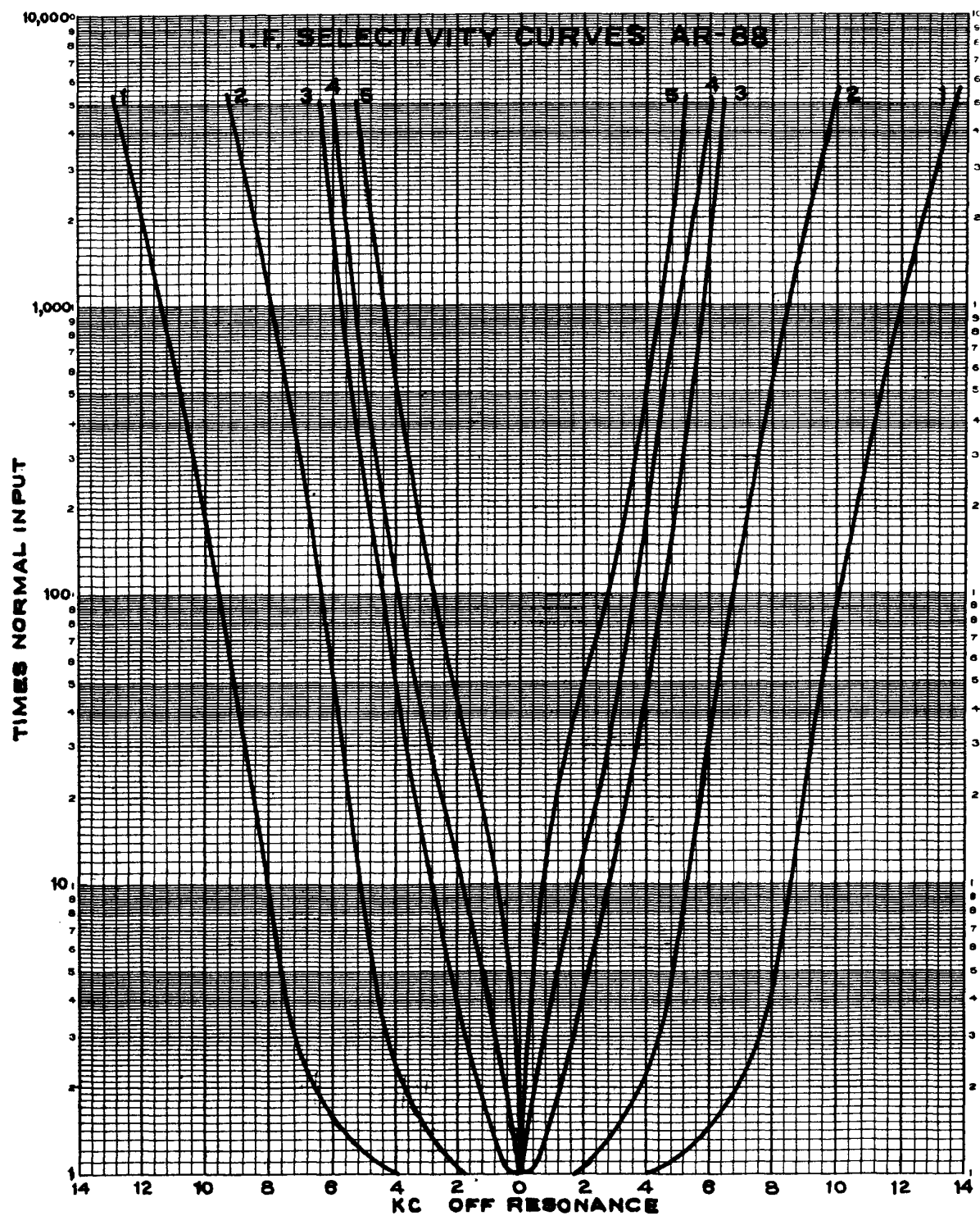
Figure 12—Selectivity Curves
