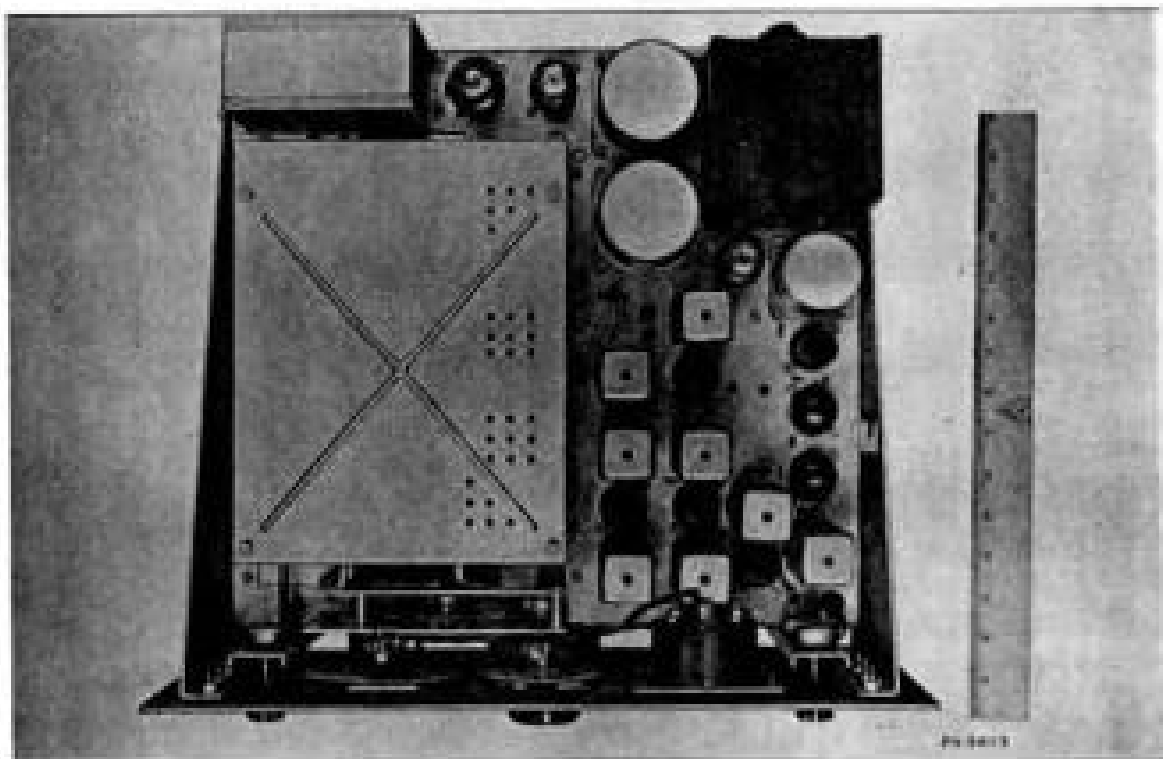
Figure 7—Top View of Chassis
