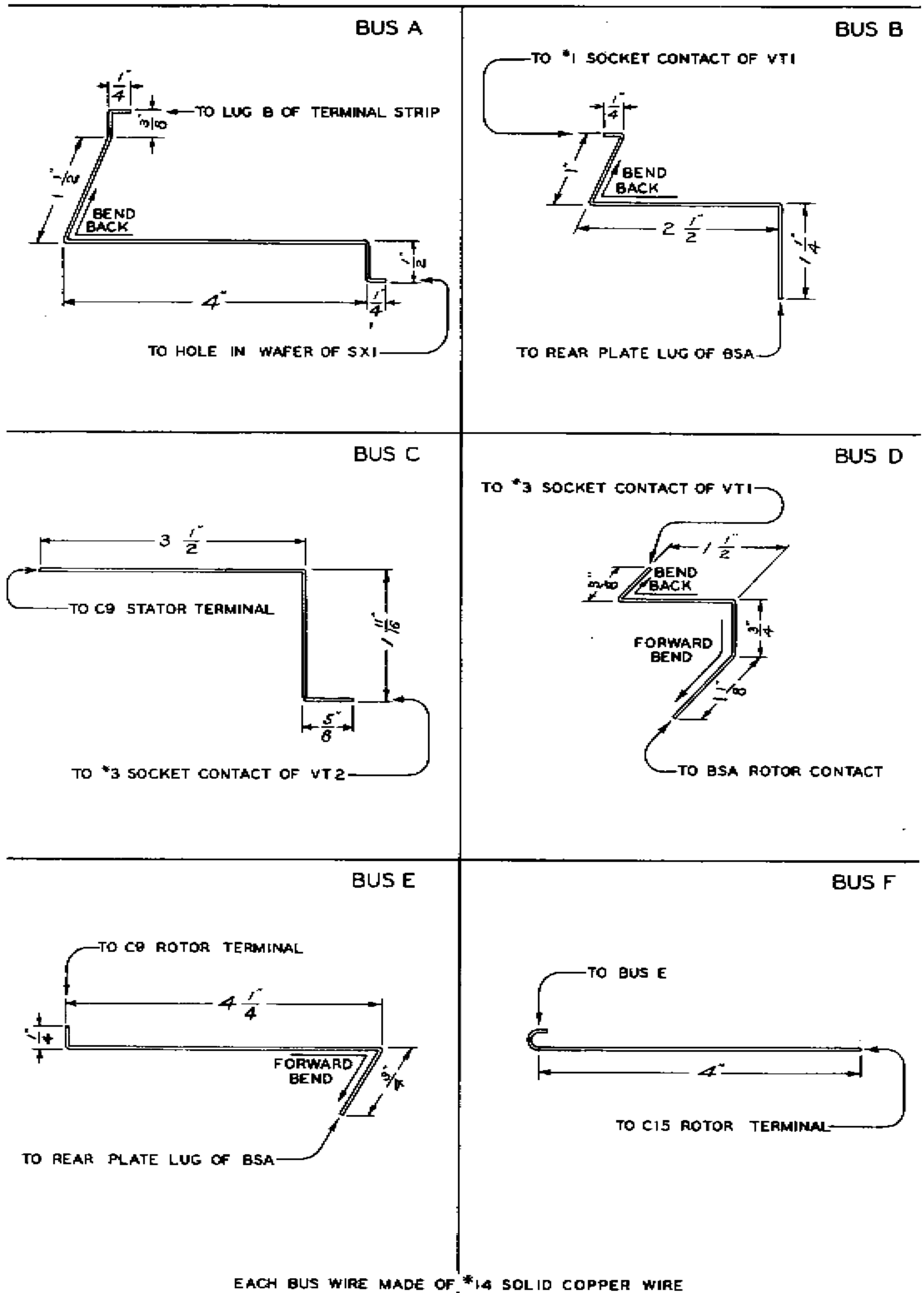
Figure 5. Formation of Bus Wires Used Below Chassis
