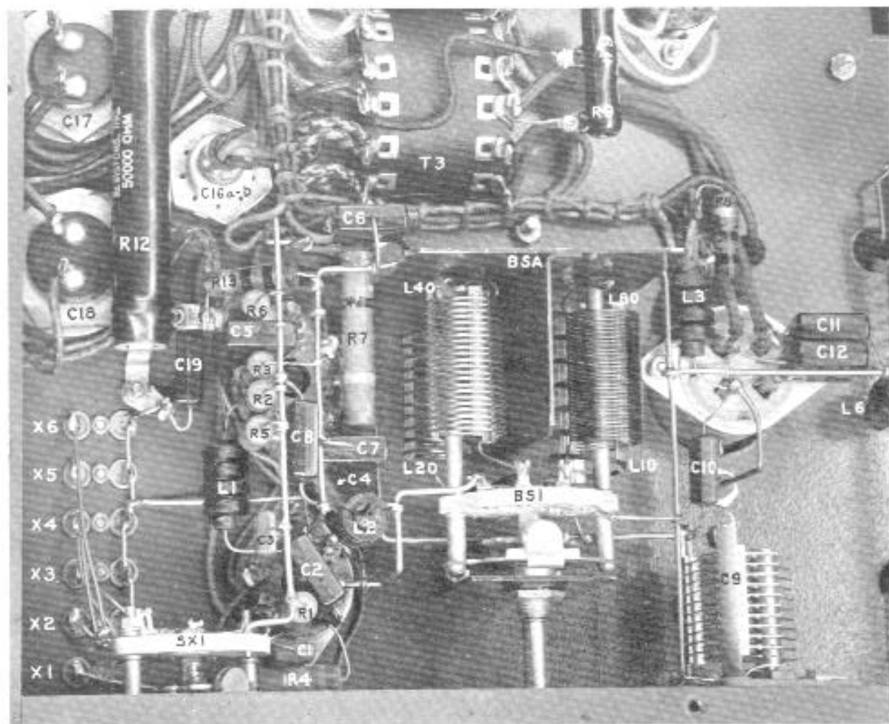
Figure 1. ST-202-A Under Chassis Close-Up
