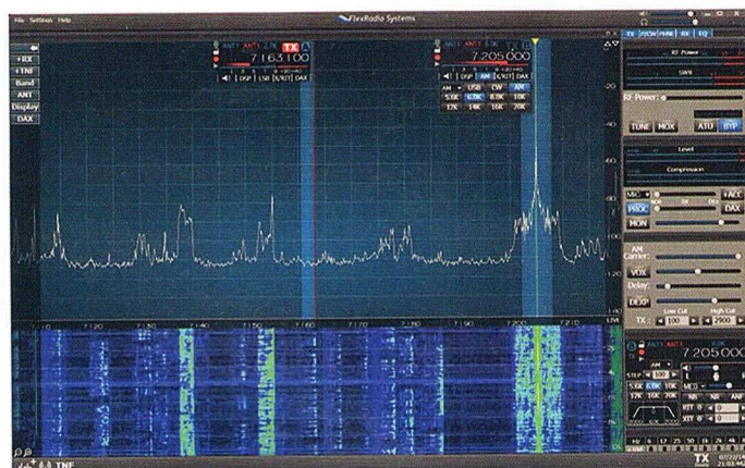
SmartSDR screen - panadapter + waterfall with 2 slice receivers. Horizontal lines on waterfall are local electric fence ticks.
