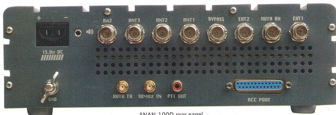
ANAN-100D rear panel.
