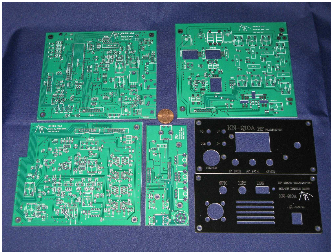
PCB's (Up left: Digital board. Up right: PA board. Down left: Analog board. Down middle: Front panel. Down right: chassis front panel and rear panel.)
