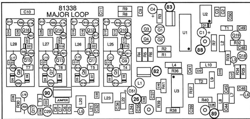
FIGURE 6-25. 81338 MAJOR LOOP BOARD COMPONENT LAYOUT
