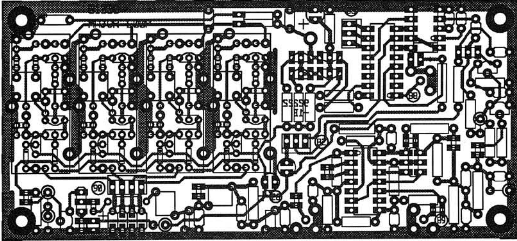
FIGURE 6-24. 81338 MAJOR LOOP BOARD CIRCUIT TRACE
