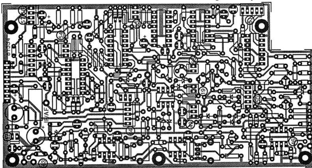
FIGURE 6-17. 81334 IF / AF BOARD CIRCUIT TRACE
