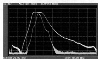
VRF Pattern (14 MHz)
