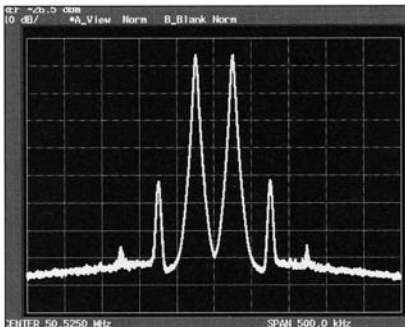
Fig. 15-2 : 50 MHz Class-A IMD Performance
