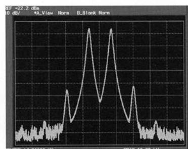
Class-A Transmitter IMD Performance (75W Output)
