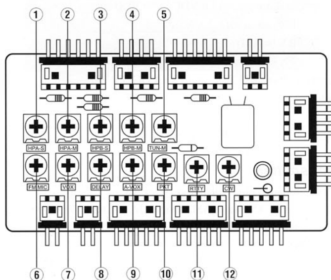
Fig. 13-1 : Top Control Panel
