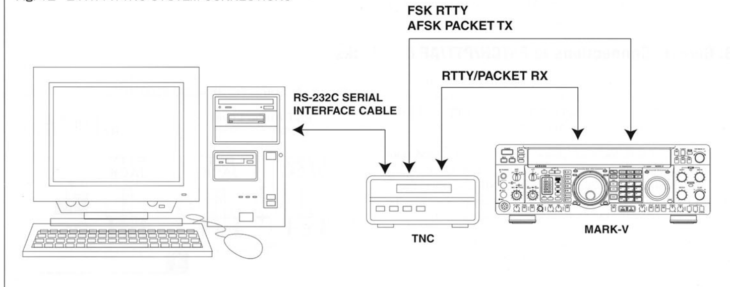
Fig. 12-2 : RTTY/TNC SYSTEM CONNECTIONS
