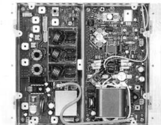
● FTV-1000 Power Amplifier Left : Low-Pass Filter Right : PA Module
