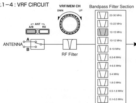
Fig.1-4 : VRF CIRCUIT
