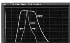
VRF Selectivity Performance (3.5 MHz)
