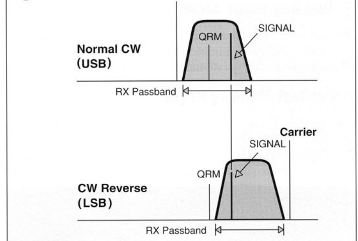
Fig. 7-3 : CW REVERSE Carrier
