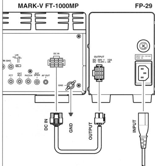
Fig. 9-1 : MARK-V/FP-29 INTERCONNECTIONS
