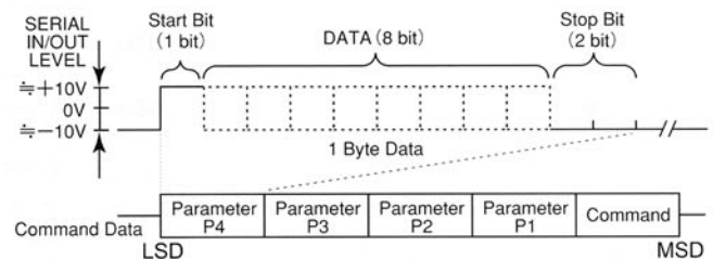
Fig. 11-1 : CAT System Data Format SPEED : 4800 bits/sec DATA BIT : 8 START BIT : 1 STOP BIT : 2 PARITY BIT : NONE
