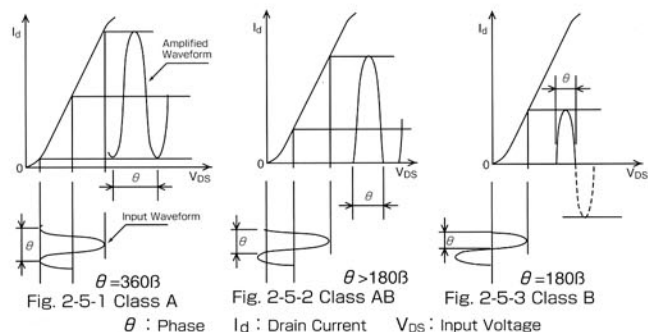
Fig. 2-5 : AMPLIFIER OPERATING CHARACTERISTICS
