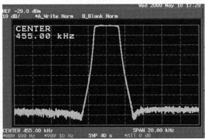
●New-technology 10-pole Collins® Mechanical Filter Skirt Selectivity
