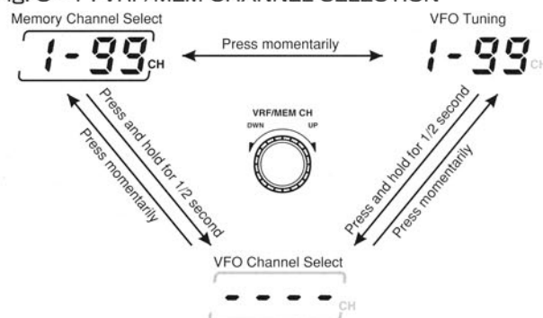
Fig. 8-1 : VRF/MEM CHANNEL SELECTION
