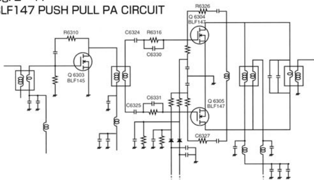
Fig. 2-4 : BLF147 PUSH PULL PA CIRCUIT
