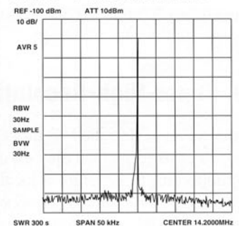
Fig. 4-1 : TX C/N RATIO
