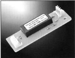
Collins® Mechanical Filter YF-115C (CW 500Hz Filter)
