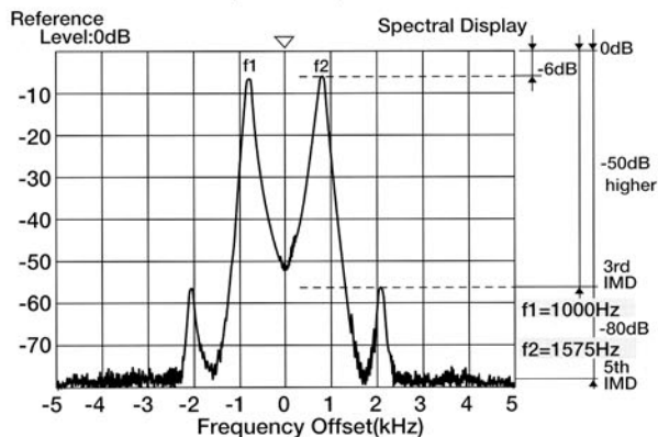
Fig. 2-8 : 2-TONE IMD (CLASS A)
