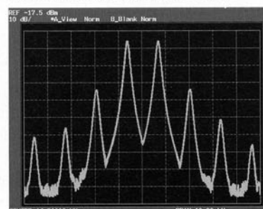
Typical Class-AB IMD at 200 W Output
