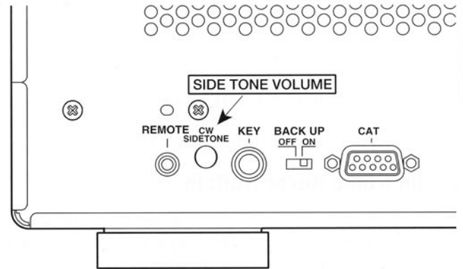
Fig. 7-5 : SIDE TONE ADJUSTMENT
