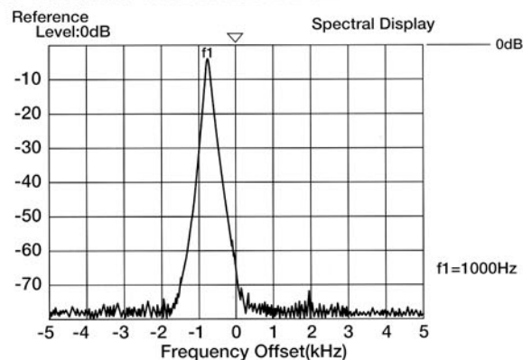
Fig. 2-6 : SINGLE-TONE SPECTRAL GRAPH
