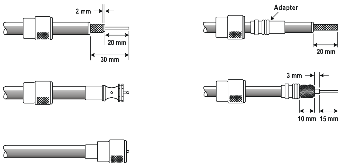
TYPICAL PL-259 INSTALLATION
