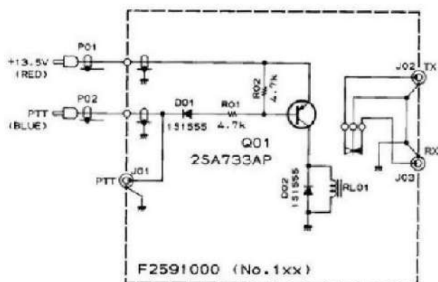
FRB - 575 CIRCUIT DIAGRAM
