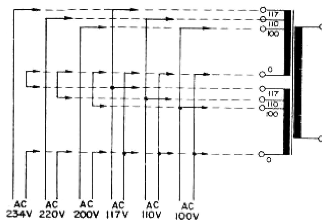
FP-757HD POWER TRANSFORMER PRIMARY CONNECTIONS
