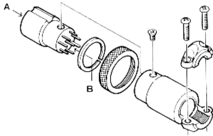
Plug assembly
