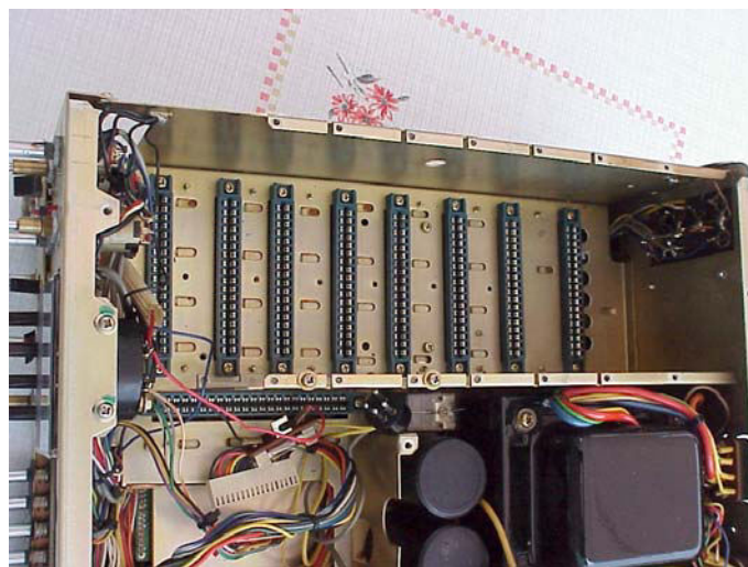
My FT-901D chassis with all modules removed for a good cleaning job
