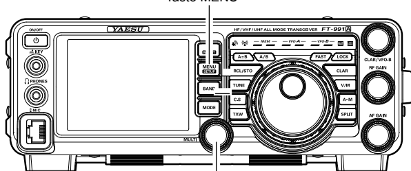
Manopola MULTI
