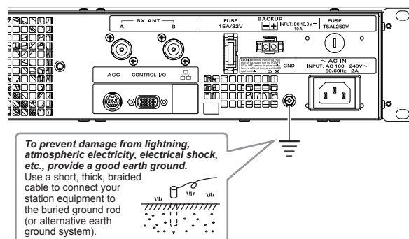
The figure above shows the rear panel of the DR-2X.
